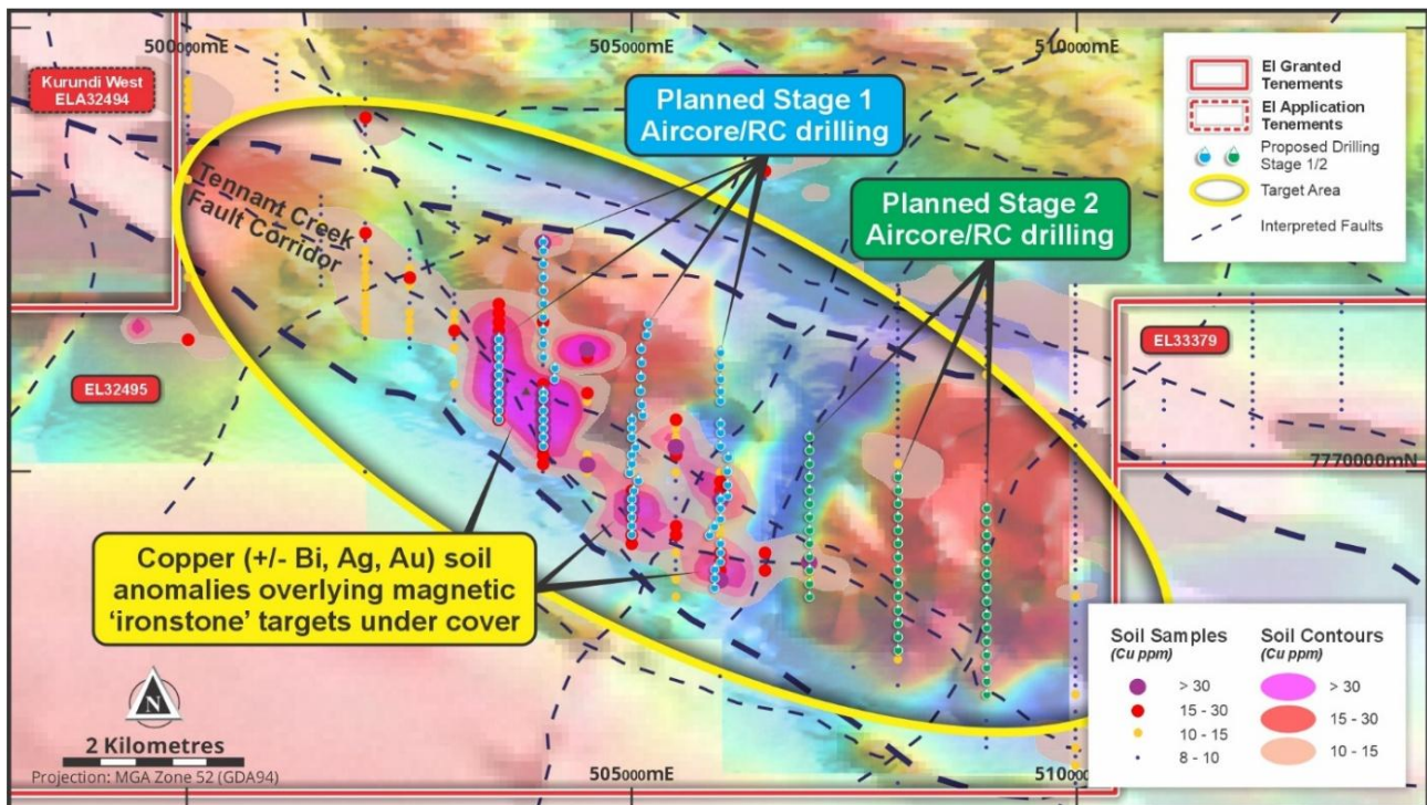
Figure 3: Kurundi North magnetic 'ironstone' targets and copper soil anomalies with planned Aircore/RC drilling
