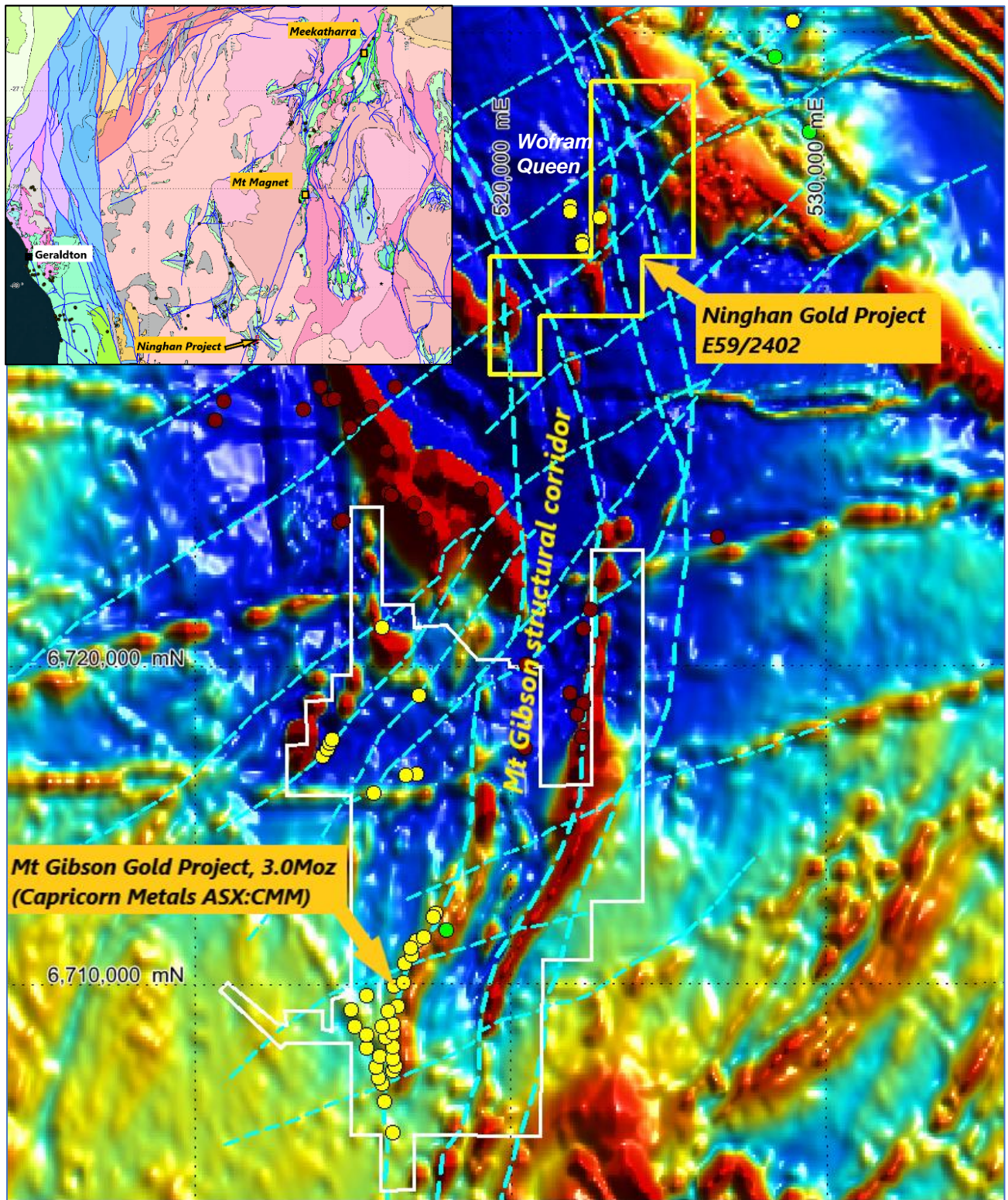
Figure 1: Ninghan Gold Project on regional magnetics image (TMI, RTP) and Mt Gibson gold deposit
