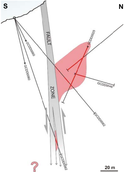
Figure 1 – Guchab cross-section (looking west) showing likely geometries in the southwest of the deposit. The mineralisation (pink) appears to be offset by faulting, and likely occurs deeper to the south. Note that the mineralisation is oblique to this section, so appears to lense out up-dip in this section.
